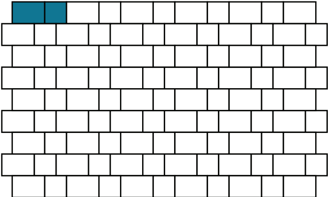
2PC. RUNNING BOND 60% 6X9 40% 6X6
